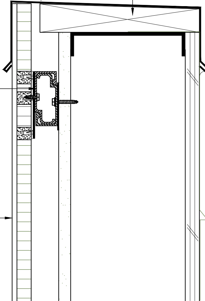
TYPICAL COPING DETAIL
